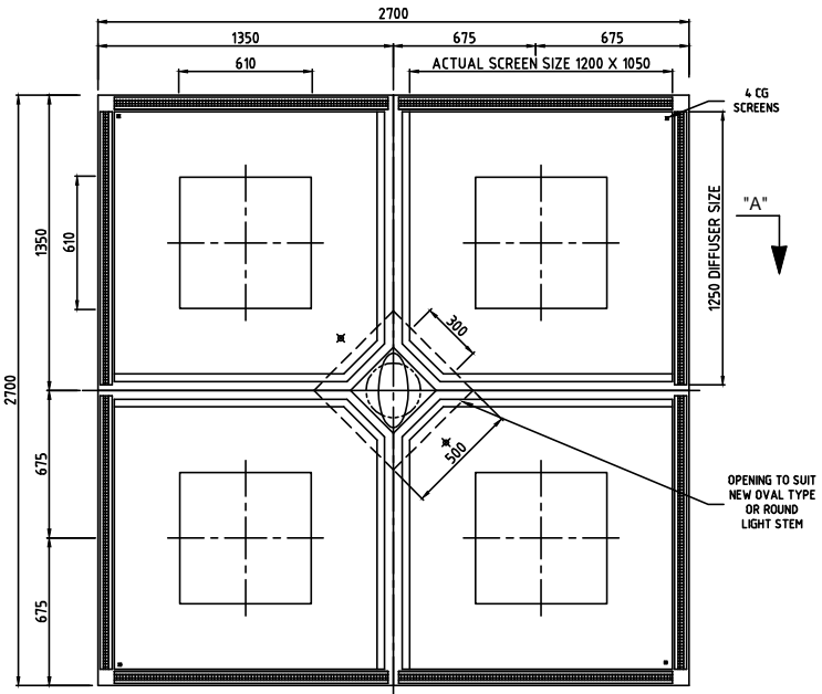
VIEW FROM UNDERNEATH PLENUM
