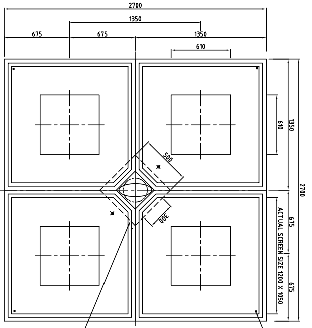
VIEW FROM UNDERNEATH PLENUM
